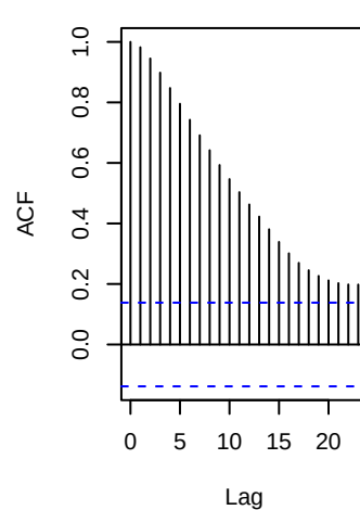
ARIMA(1,1,0) ACF
