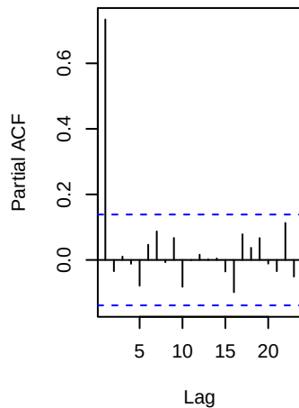
ARMA(1,1) PACF
