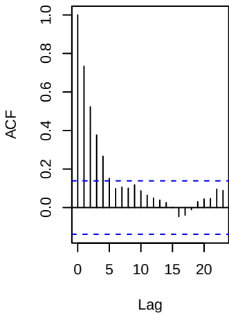
ARMA(1,1) ACF
