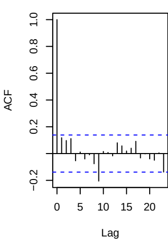
ARMA(1,1) ACF
