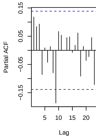
ARMA(1,1) PACF
