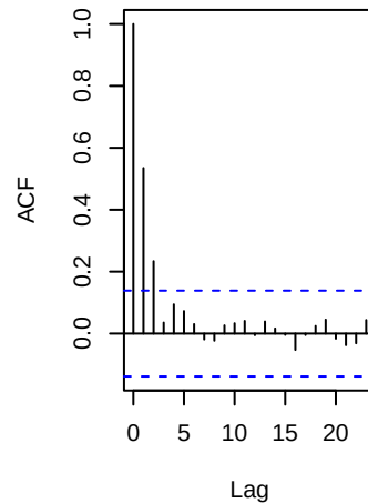
ARIMA(1,1,0) ACF
